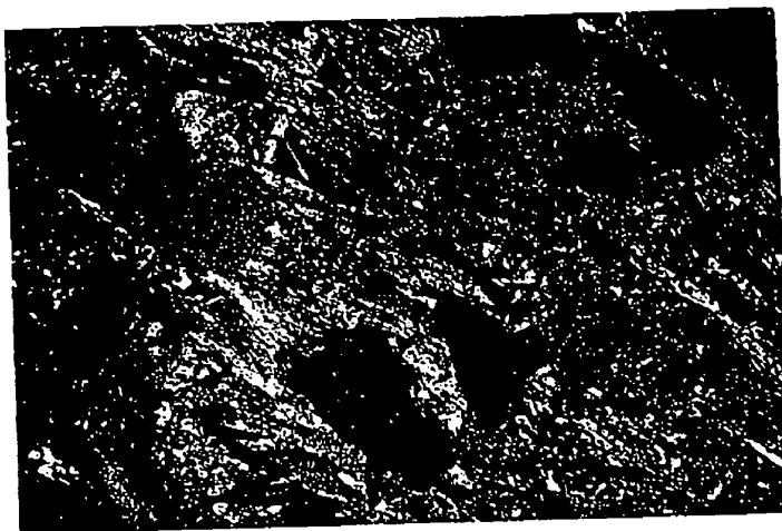
Fig. 2b. Photomicrograph, magnification \times 24 , of thin section V 2 under XN showing areas of coarse lamellar talc intergrown with fine grained talc-serpentine aggregates and enclosing anhedral grains of magnesite.
