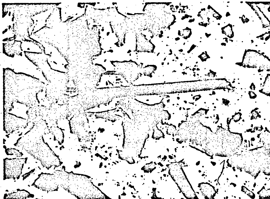
Fig. 13 Specimen I41. Face 2, good talc specimen x 3000. Plate-like particles together with rolled talc sheets lath forms and textile type fibres.
