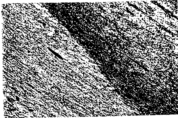
Fig. 11d. Photomicrograph, x 40 mag., of thin section V 11B under XN showing the interlaminated chlorite (white) in talc (displaying range of interference colours), and the transgressive nature of the boundary between the 'dusty' and clear talc.
