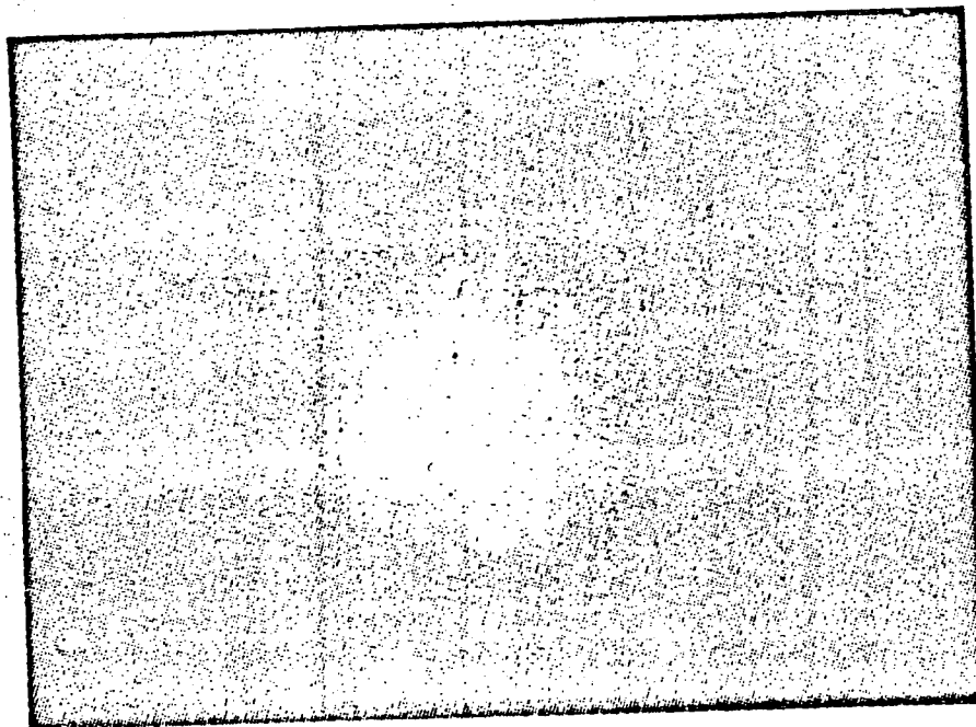
Amphibole asbestos selected area electron diffraction pattern.
