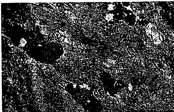
Fig. 2a. Photomicrograph, magnification x 24, of thin section V 2 under PPL showing grains of anhedral magnesite in a compact coarse to fine grained talc matrix.
