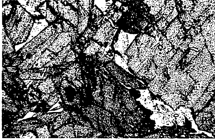
Fig. 9a. Photomicrograph, x 24 mag., of thin section V 9 under PPL displaying coarse actinolite with minor interstitial talc.
