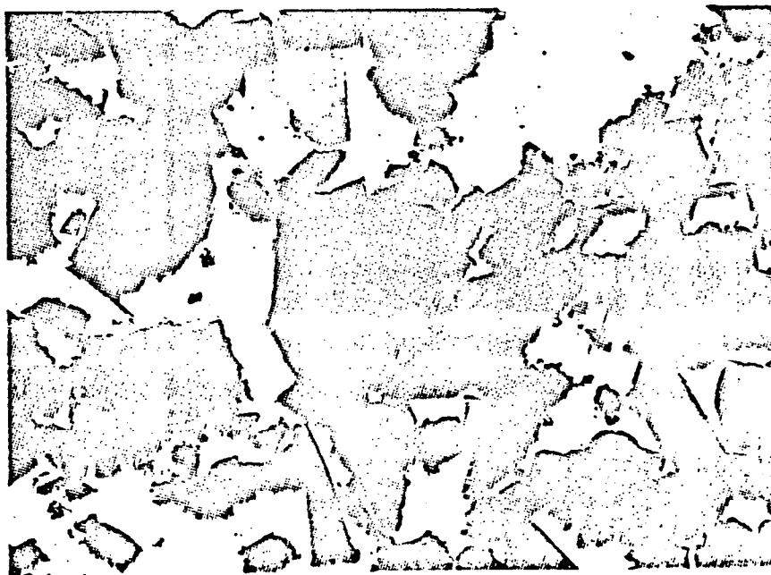
Fig. 16. Specimen I44. Face 1. Pure talc sample, x3000. Plate-like particles with some lath-like forms.
